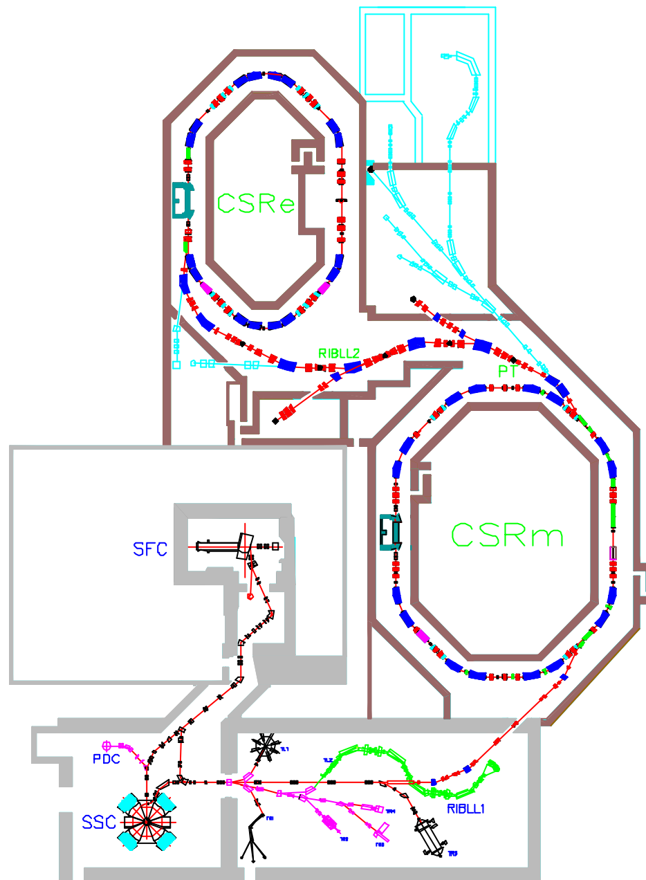
Overall Layout of HIRFL-CSR
